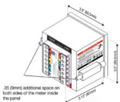
PowerLogic™ PM1000 series power meter dimensions and DM6000 series digital panel meter dimensions
