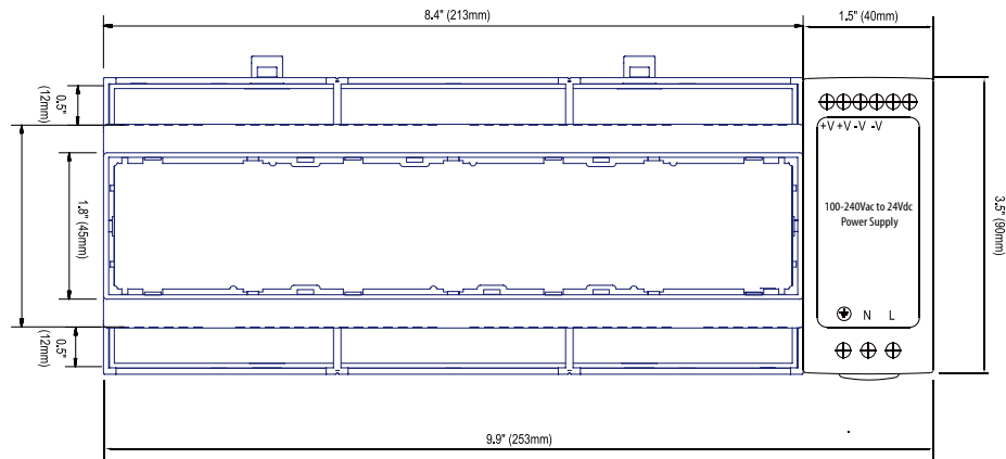
Figure 1 - Top View
