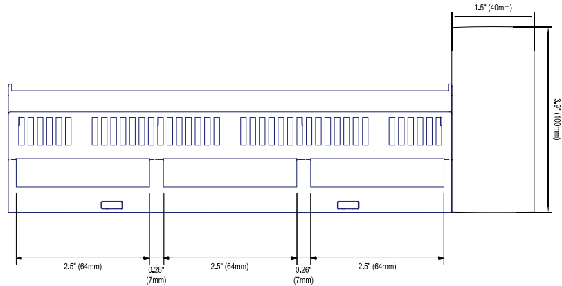
Figure 3 - Front view
