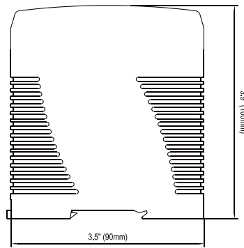
Figure 4 - Side view of Power Supply unit
