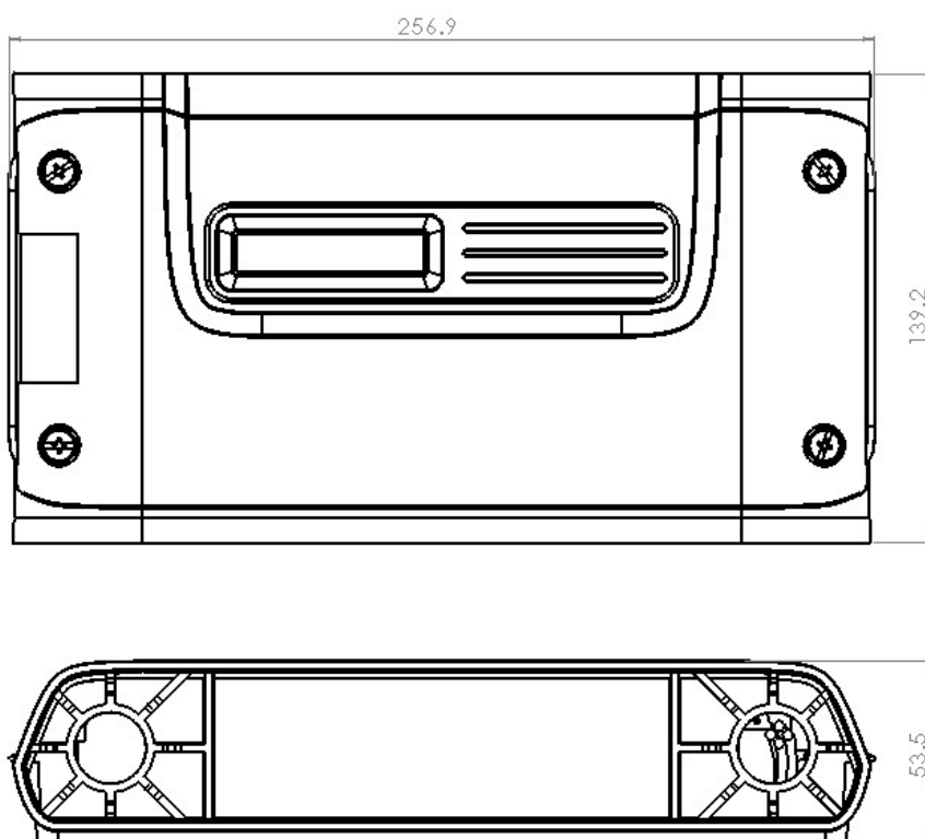
PS3HD Wall Mount Enclosure Dimensions
