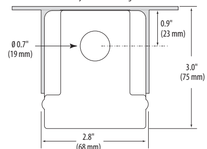
Removable/Adjustable Mounting Bracket
