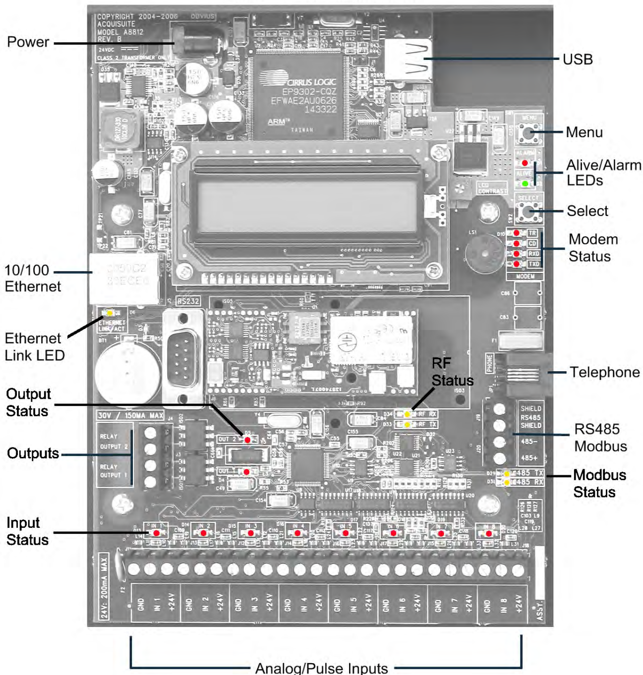
AcquiSuite A8812 Internal View
