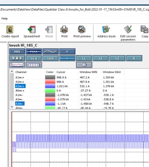
Display InRush peak.
